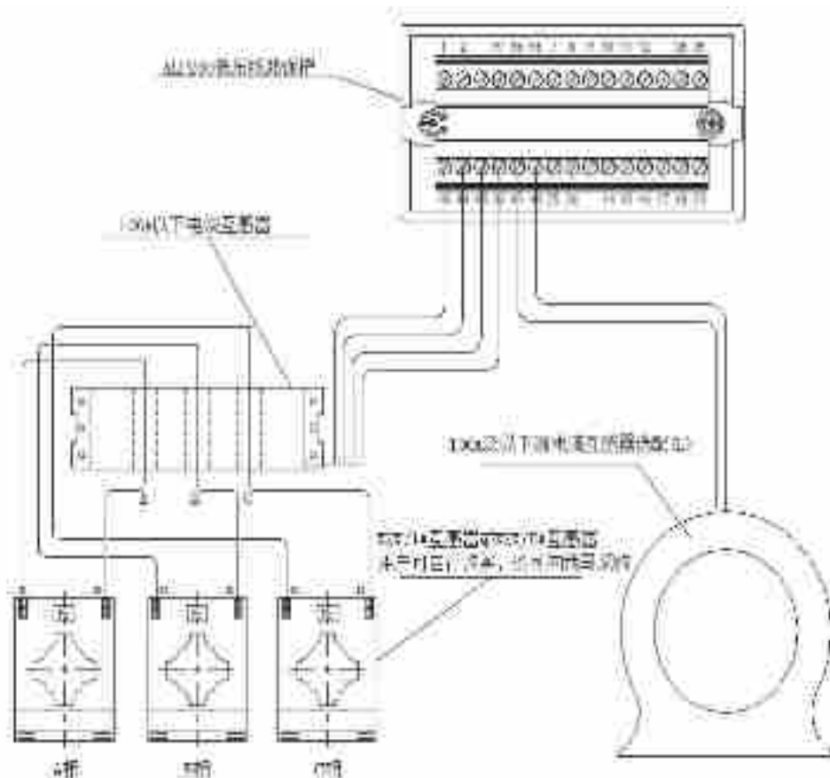
图 12 ALP200-1A、ALP200-5A 产品组成 Figure 12 Product composition of ALP200-1A, ALP200-5A
